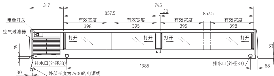
HNC-210BC-R-B
